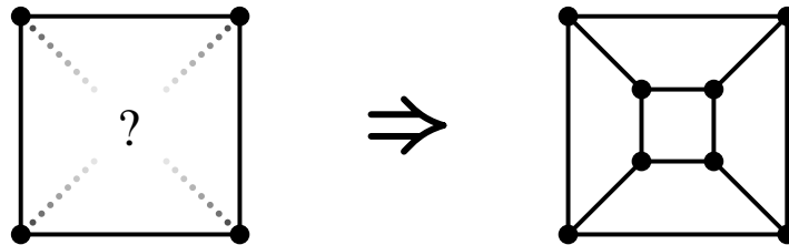
Figure 2: Tutte Embedding (TE) of the graph of a cube projected onto the plane.
