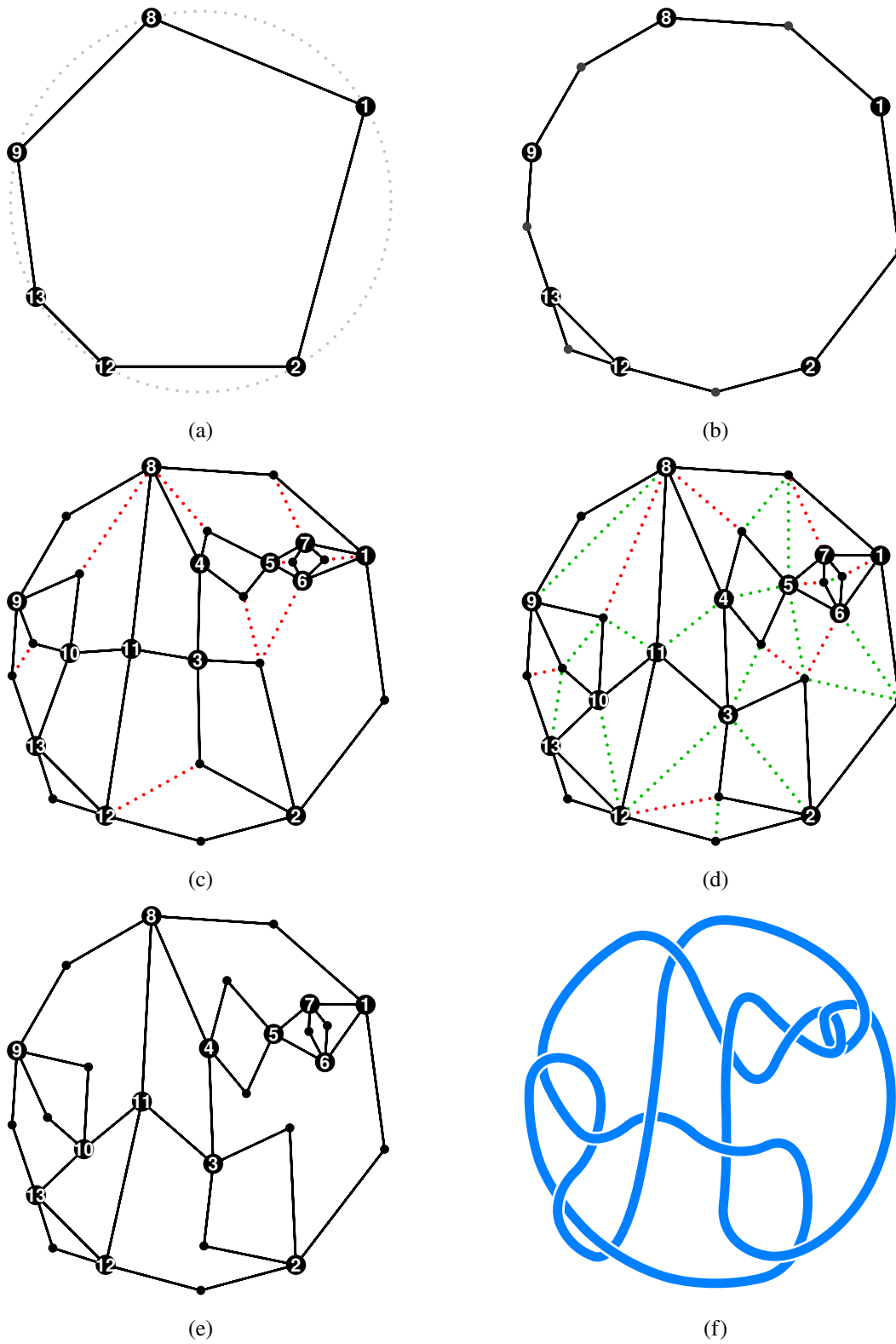
Figure 8: Embedding 13ah_1131: (a) bounding polygon, (b) perimeter splitting, (c) TE after augmentation, (d) TE after triangulation, (e) virtual edges removed, and (f) drawn without smoothing.
