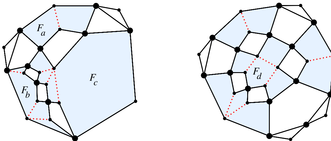
Figure 6: Virtual edges (dotted lines) augment these graphs to achieve internal triconnectivity.
