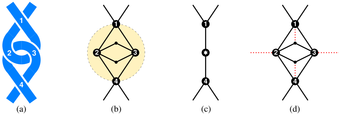
Figure 4: Vertices 1 and 4 form a separation pair whose disconnected set will collapse unless augmented.
