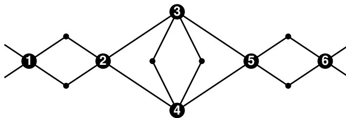
Figure 5: This structure of linked separations has two separation groups represented by (1, 6) and (3, 4) .
