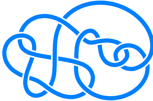
Figure 7: Smoothed drawing of Regina knot 13ah.1131.
