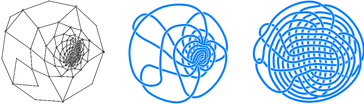
Figure 9: 138-crossing projection of the unknot embedded (left), drawn (middle) and smoothed (right).
