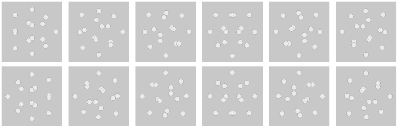
Figure 7: 12 frames that form an animated loop of the juggling pattern (3, 8, 15) . Notice that because of the symmetries of the underlying pattern, there are only two distinct configurations of points in these 12 frames; a bilaterally symmetric configuration appears in four rotations, and an asymmetric configuration appears in eight rotated and reflected orientations.
