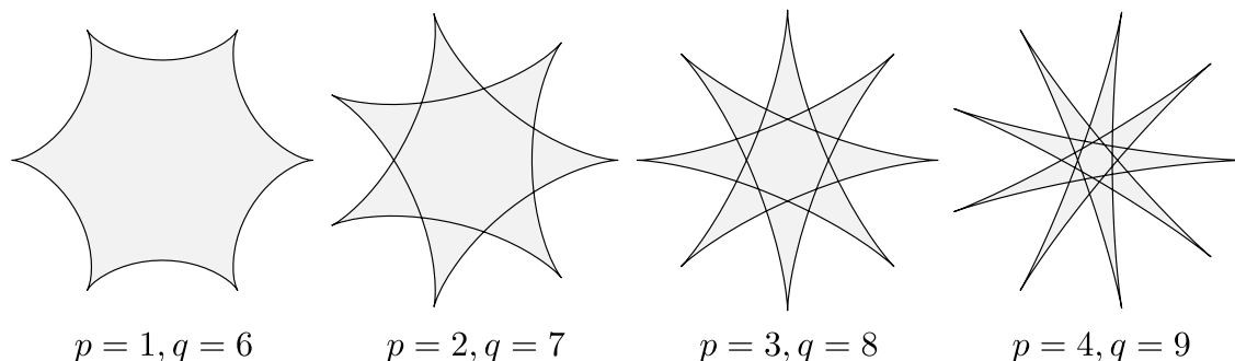
Figure 2: Drawings of a few simple rational hypocycloid curves based on gears of radius p/q rolling around the inside of a unit circle.
