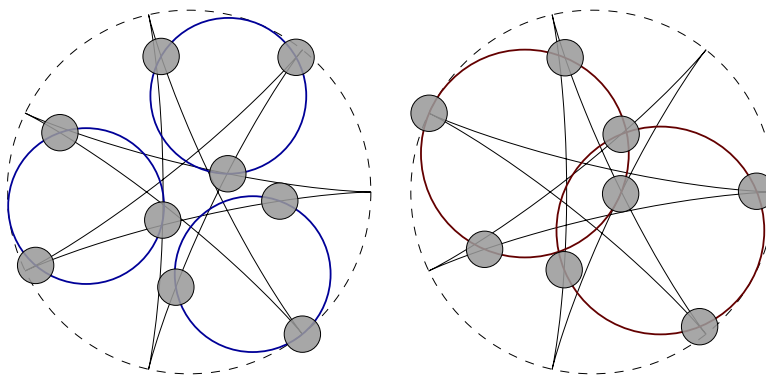
Figure 4 : Two different juggling patterns with different groupings. On the left, the pattern (3, 7, 9) decomposes into three primary wheels of three points each and no secondary wheels. On the right, the pattern (3, 7, 8) decomposes into two secondary wheels of four points each and no primary wheels. In this figure and in Figure 6, the wheels are visualized using circles instead of regular polygons, in order to emphasize their connection to the underlying hypocycloid.
